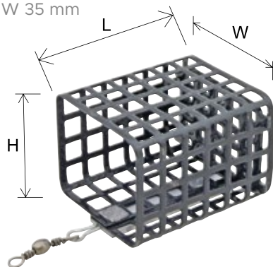
Block End Steel Feeder "Square"
